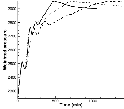
FIGURE 10. Weighted pressure in the entire domain for the second order formulation using an equivalence ratio of 0.3 (CFL 0.5 ..... ; CFL ramp from 0.5 to 2.0 ---- ; CFL ramp from 0.5 to 3.0 — ).
