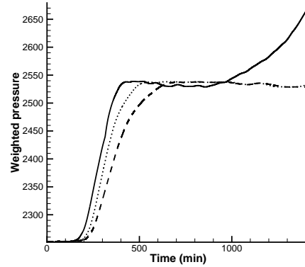
FIGURE 15. Weighted pressure convergence for equivalence ratio of 0.4, and second order method (CFL 0.5 ..... ; CFL ramp from 0.5 to 1.5 ---- ; CFL ramp from 0.5 to 2.0 ———).
