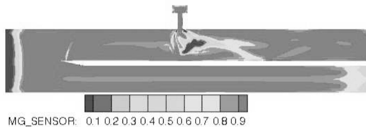
FIGURE 3. Visualization of the pressure and viscous sensors during a multigrid simulation of a jet in cross flow.
