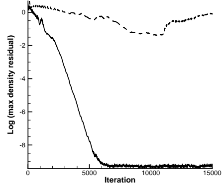
FIGURE 7. Effect of the new boundary Jacobian, and time step evaluation in the convergence of the hypersonic (2nd-order) flow around a cylinder (old formulation --- ; new formulation --- ).
