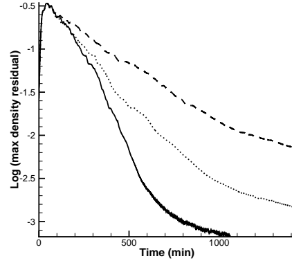
FIGURE 9. Residual convergence of the second order Hyshot simulation using an equivalence ratio of 0.3 (CFL 0.5 ..... ; CFL ramp from 0.5 to 2.0 ---- ; CFL ramp from 0.5 to 3.0 _____).
