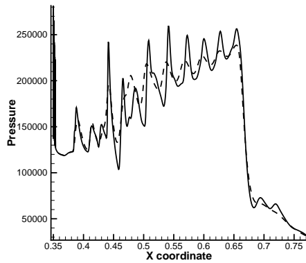
FIGURE 12. Pressure distribution on the body wall of the scramjet using a second (—) and a mixed method (----).
