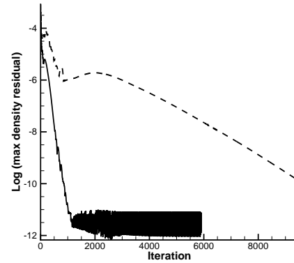
FIGURE 2. Subsonic laminar flow around a NACA0012 (single grid --- ; 4MG levels — ). First level 16000 hexahedra 1:4 reduction. 64230 faces. Speed up to residual level of 10^{-6} x9 (iterations)
