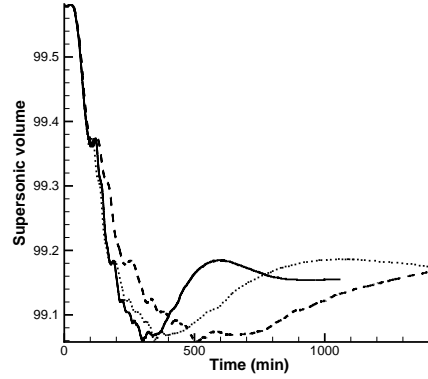
FIGURE 11. Supersonic flow percentage in the entire domain for the second order formulation using an equivalence ratio of 0.3 (CFL 0.5 ..... ; CFL ramp from 0.5 to 2.0 ---- ; CFL ramp from 0.5 to 3.0 — ).
