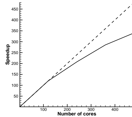
FIGURE 13. Scalability study of the Hyshot II reacting simulation (Joe scalability — ; linear scalability ----).
