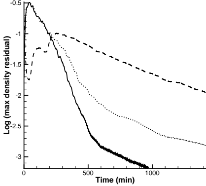
FIGURE 8. Residual convergence of the mixed order Hyshot simulation using an equivalence ratio of 0.3 (CFL 0.5 ..... ; CFL ramp from 0.5 to 2.0 ---- ; CFL ramp from 0.5 to 3.0 _____).
