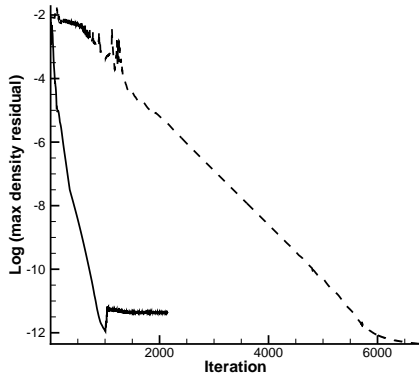
FIGURE 1. Supersonic flow around a cylinder (single grid --- ; 5MG levels — ). First level 16384 hexahedra 1:4 reduction. 65856 faces. Speed up to residual level of 10^{-4} x17 (iterations)
