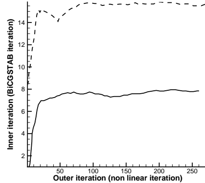
FIGURE 5. Effect of the preconditioning on a RANS simulation (Reynolds number 6.5 \cdot 10^6 ). Linelet preconditioner (——) versus Jacobi preconditioner (----), the convergence criteria is 0.1.
