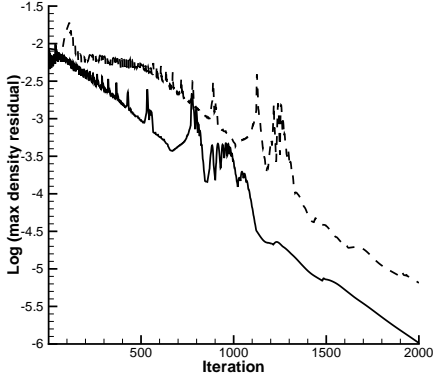
FIGURE 6. Effect of the new boundary Jacobian in the convergence of the hypersonic (1st-order) flow around a cylinder (old formulation --- ; new formulation --- ).
