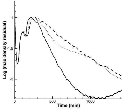
FIGURE 14. Residual convergence for equivalence ratio of 0.4, and second order method (CFL 0.5 ..... ; CFL ramp from 0.5 to 1.5 ---- ; CFL ramp from 0.5 to 2.0 ———).
