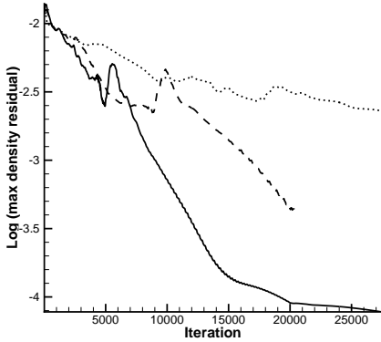
FIGURE 4. Convergence of the jet in cross flow problem: the multigrid methodology produces a speed up of 4\times (single grid ..... ; 3V MG, damping factor 0.75 ---- ; 3V MG, damping factor 0.25 ———).
